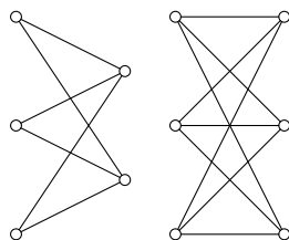
Obr. 9.9: Grafy K_{3,2} a K_{3,3}
