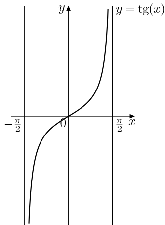
Figure: Bijekcia medzi (-\frac{\pi}{2}, \frac{\pi}{2}) a \mathbb{R}
